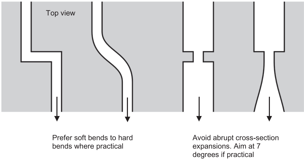
Figure 8: Reducing the turbulence and risk of scour
