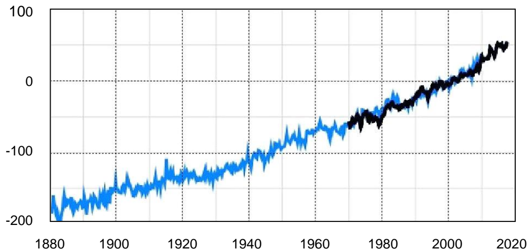
Figure 2: Global sea level rise since 1880
