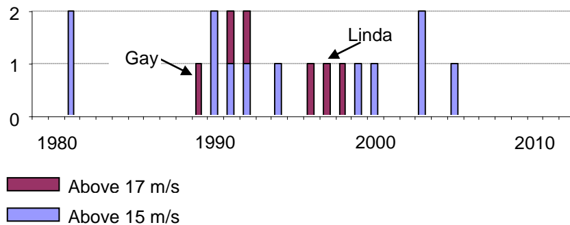
Figure 4: Occurrence of wind speeds above 15 and 17 m/s off the coast of Cambodia
