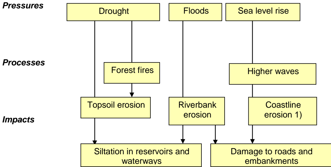
Figure 8: Climate-related causes and effects affecting infrastructure
