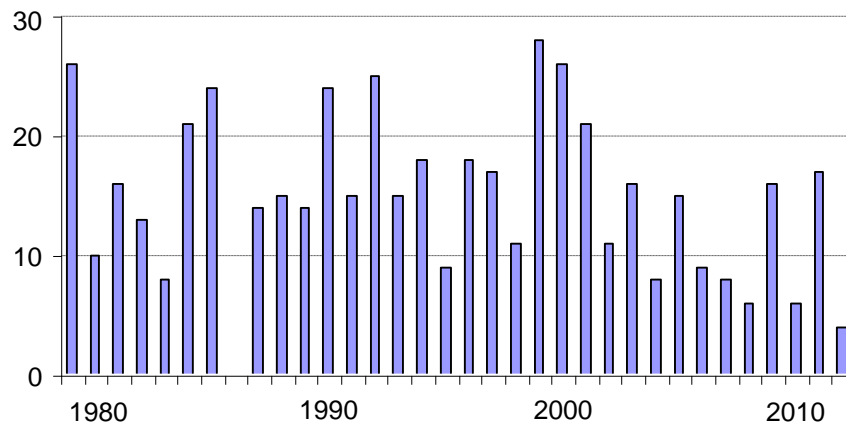
Figure 3: Occurrence of wind speeds above 12 m/s off the coast of Cambodia
